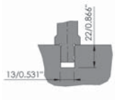
Tool slot to suit for NS V and NS IV adaption
