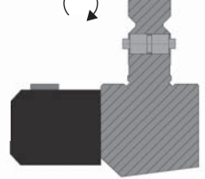
Additional roller bearing for large Gooseneck tools equipped with E2M®. (NS I + II)
