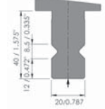
NS III New Standard II adaption
