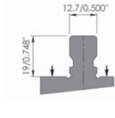
AS II American Style II adaption
