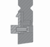
Safety-Click® Applicable for tool weight up to 12.5 kg/28 lbs. (NS I + II + AS II)
